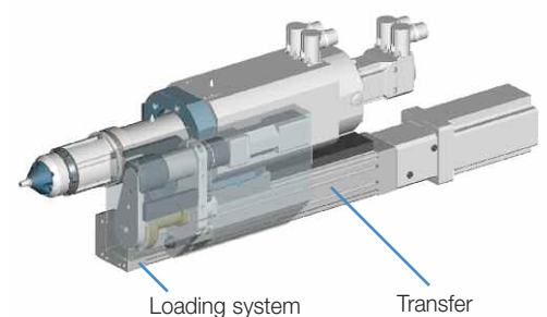
Blow feed configuration
